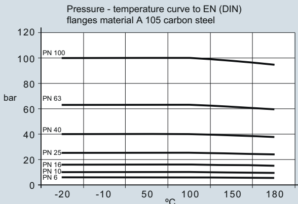
Pressure/temperature curve to EN (DIN) flanges, material A 105 carbon steel
